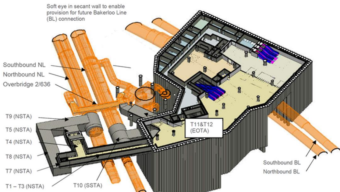
Figure 2: Core scope of new station box and connecting tunnels (shown in grey) to be constructed under the shopping centre redevelopment.
